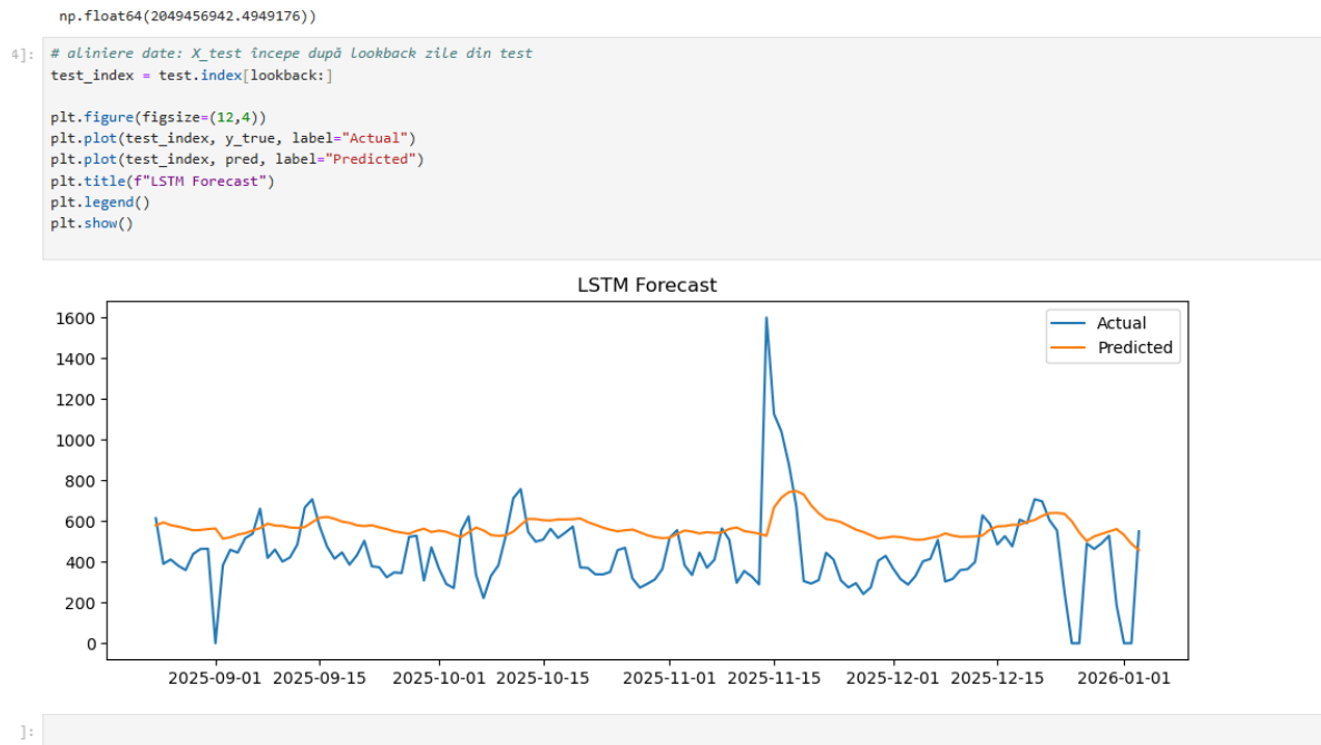
Fig. 7 LSTM Predicted
