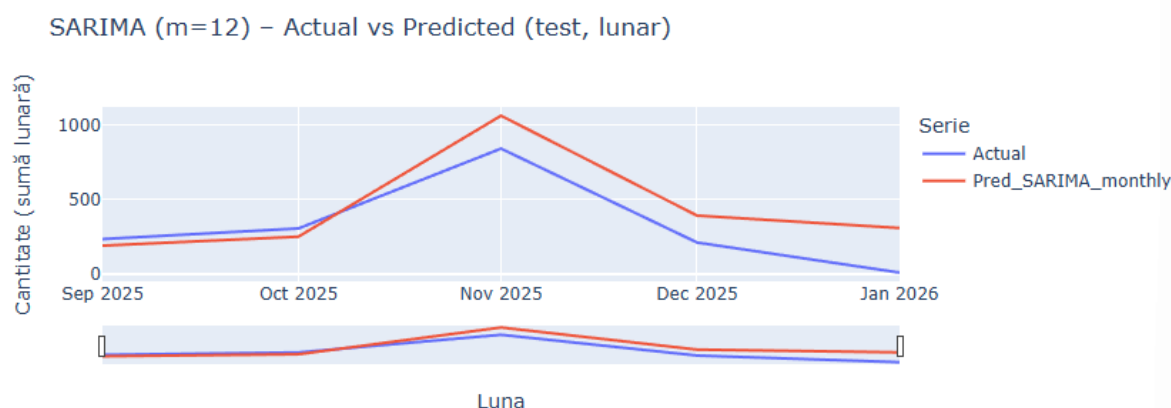
Fig. 5 Model lunar SARIMA
